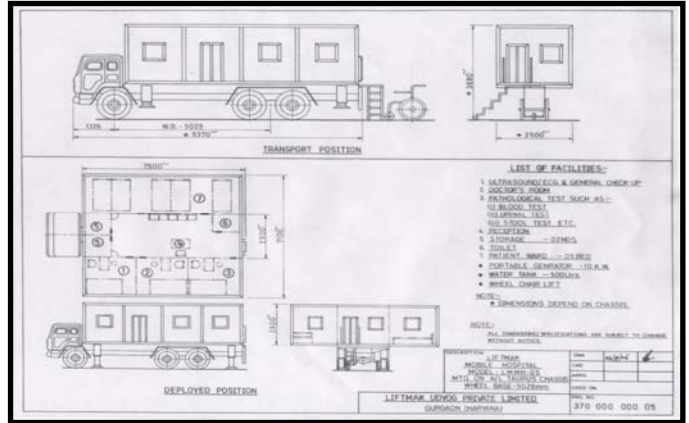
Drawing of mobile hospital with e-x-p-a-n-d-a-b-l-e body
